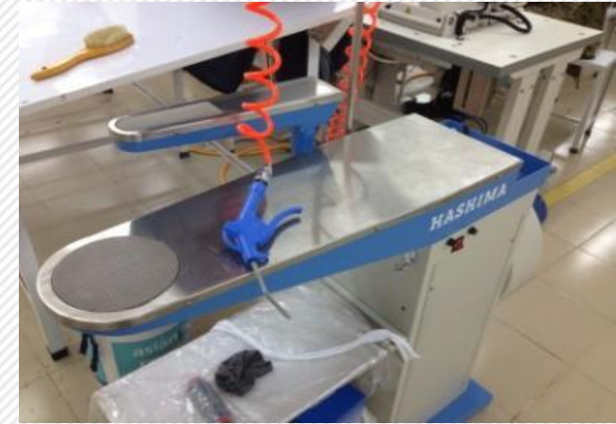
Spot removemachine
